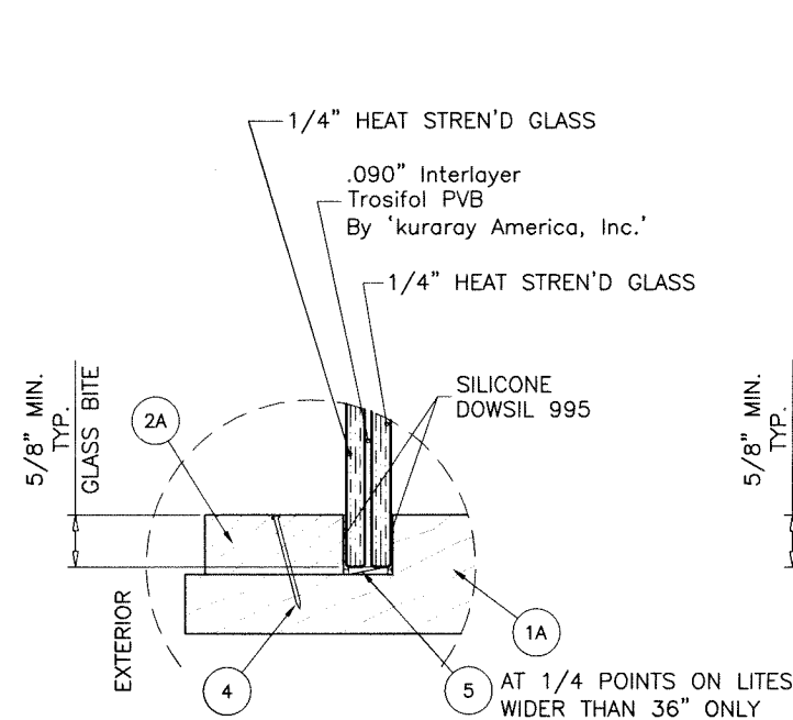
GLASS TYPE 'A' 9/16" OVERALL LAM. GLASS
