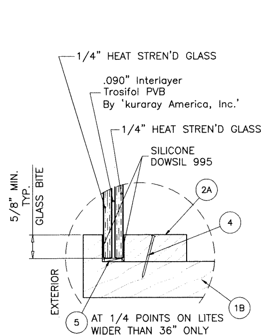
GLASS TYPE 'A' 9/16" OVERALL LAM. GLASS
