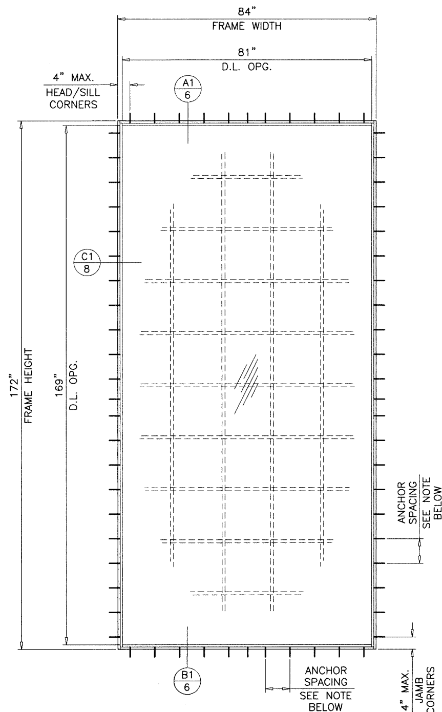
TYPICAL ELEVATION (1-1/2" FRAMES)
