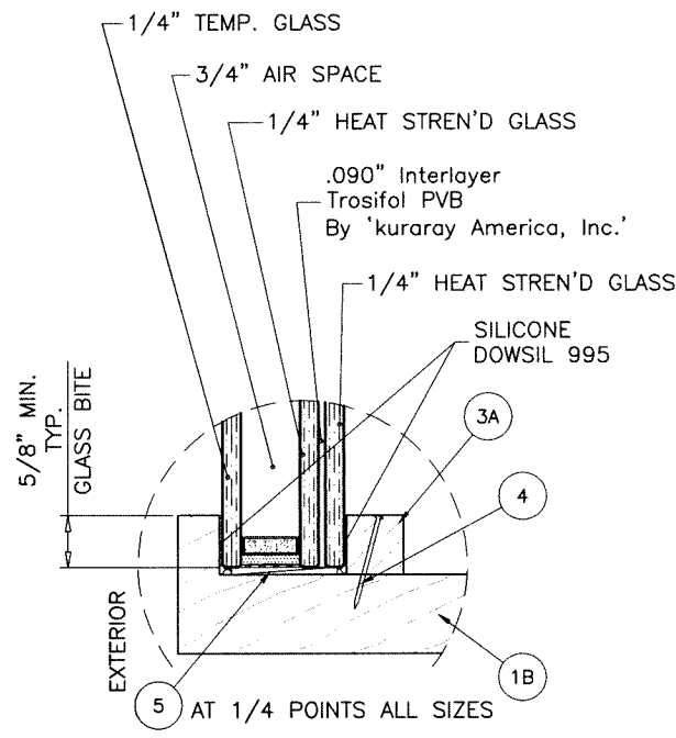
GLASS TYPE 'Ai' 1-1/2" OVERALL INSUL. LAM. GLASS
