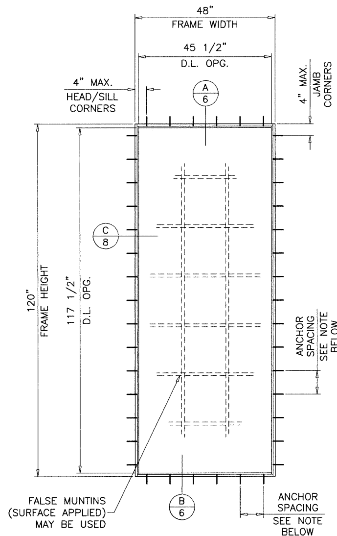
TYPICAL ELEVATION (1-1/4" FRAMES)
