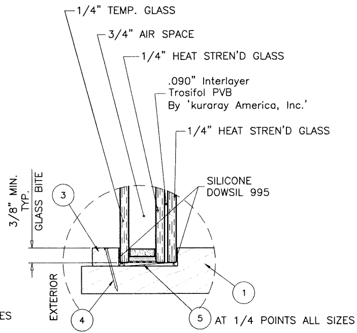
GLASS TYPE 'Ai' 1-1/2" OVERALL INSUL. LAM. GLASS
