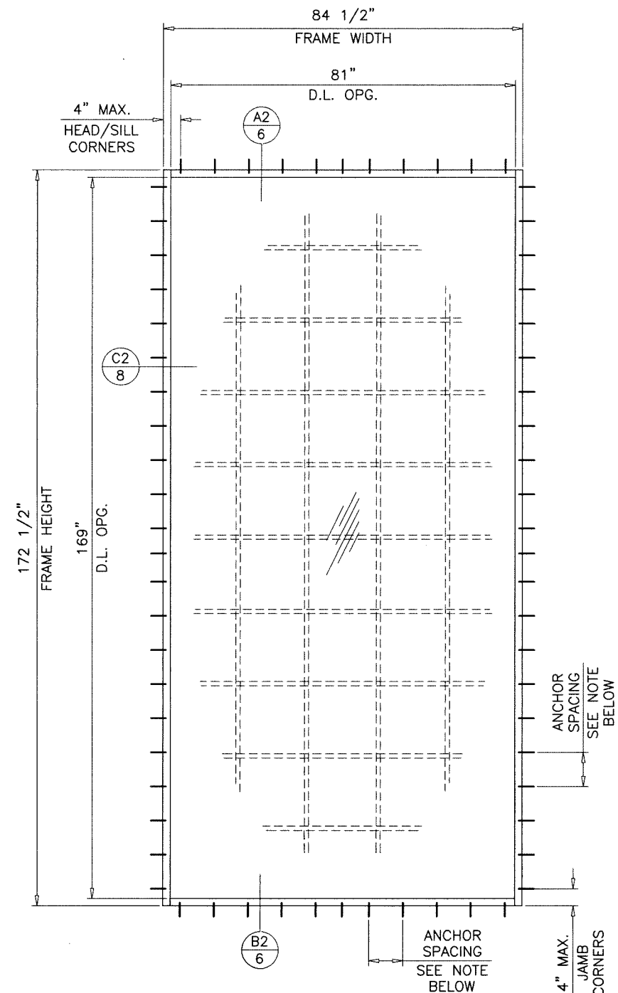
TYPICAL ELEVATION (1-3/4" FRAMES)
